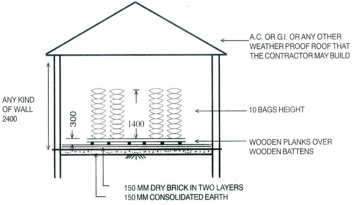
SECTION AB
