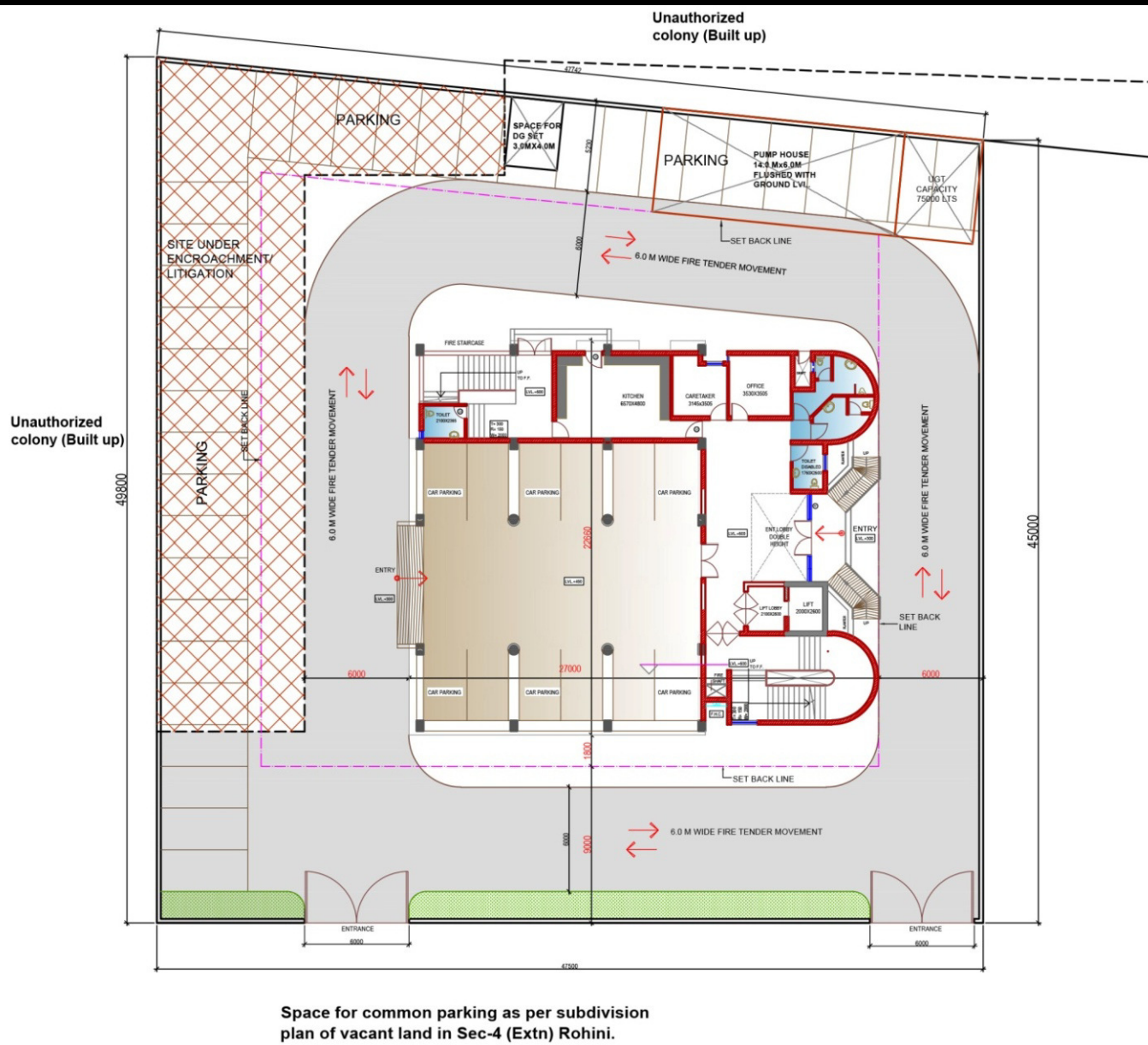
LAYOUT PLAN
