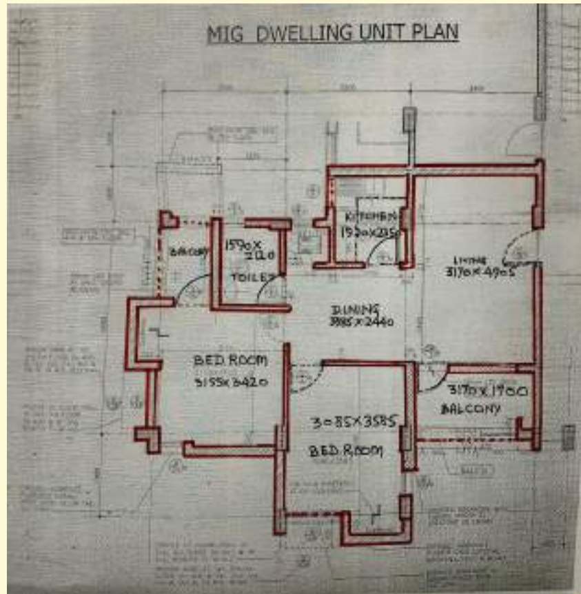
TYPICAL UNIT PLAN OF MIG (2 BHK) FLATS AT VASANT KUNJ
