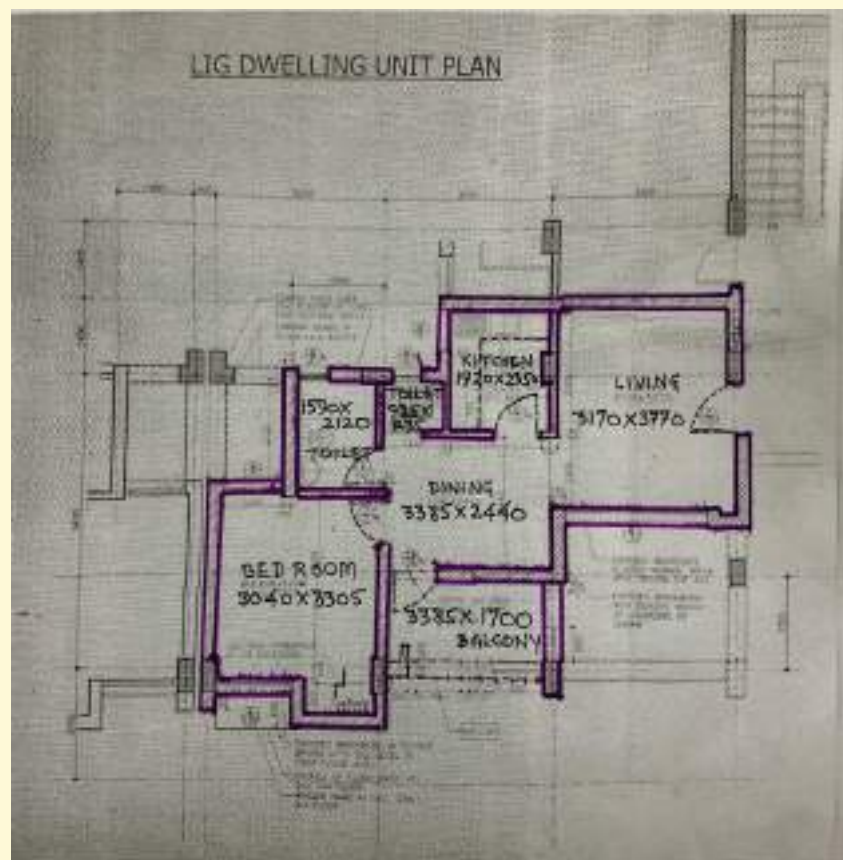
TYPICAL UNIT PLAN OF LIG (1 BHK) FLATS AT VASANT KUNJ
