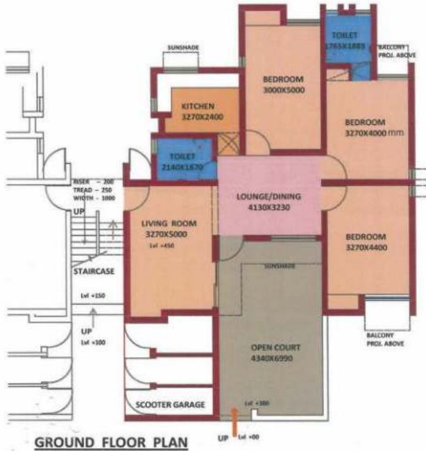
UNIT 1 – CATEGORY III Area – 109.5 sqm (approx.)
